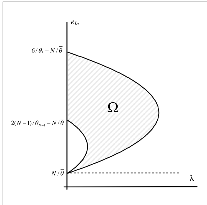
Figure 1. Set of (\lambda, e_{In}) compatible with divided organizations.
